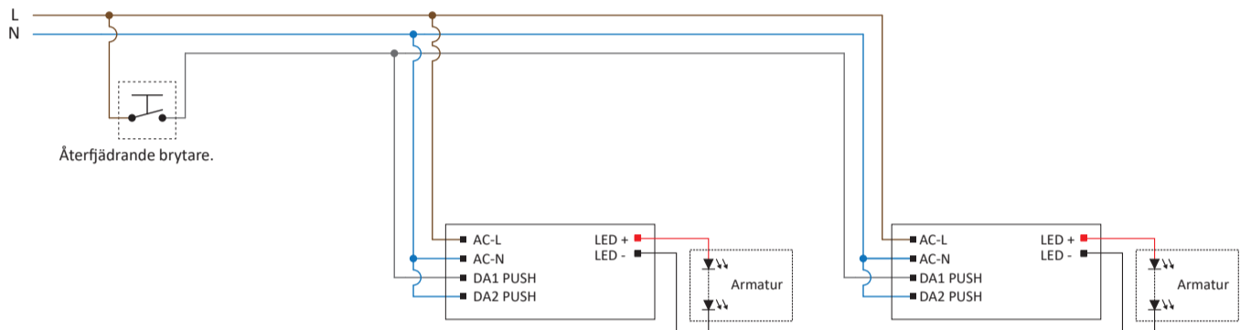
Kopplingschema Push-Dim
